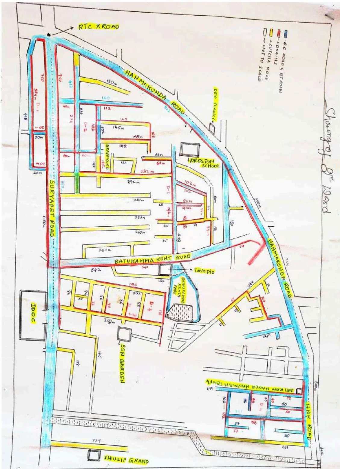
Figure 2.1 — Ward 2: Road, drain and kutchra-road network (hand-drawn, not to scale)
